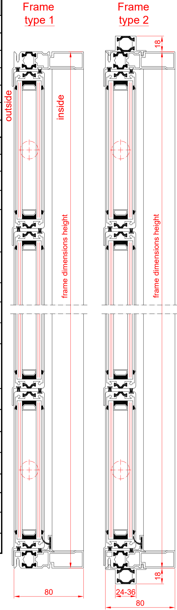
Detail frame
