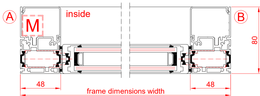
Frame type 1
