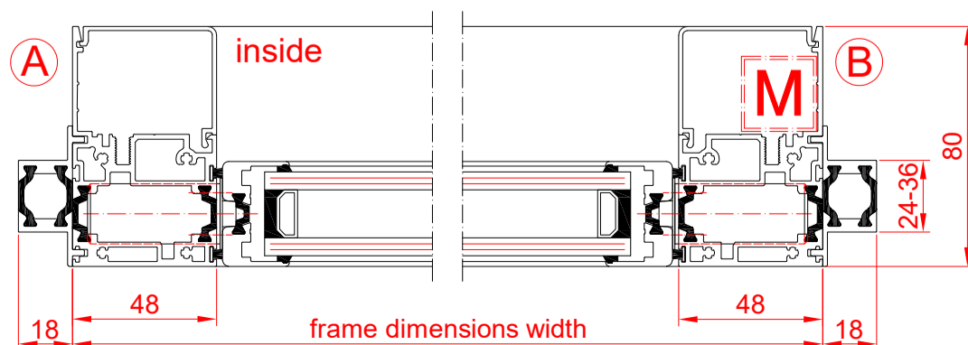
Frame type 2
