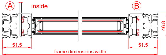
Frame type 1
